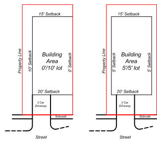
Typical Lot Setbacks Unless noted on plan
